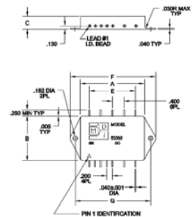
CASE STYLE 8 Seam Welded Chassis Mount with Flange
