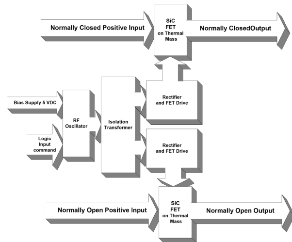
300V/5A Solid State Relay Model 53817
