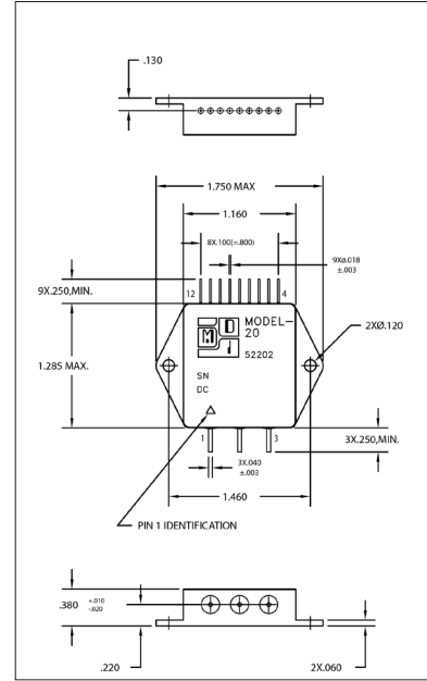
Case Style 20
