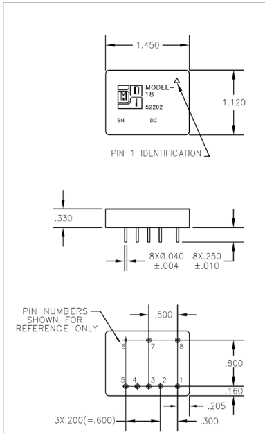
Case Style 18
