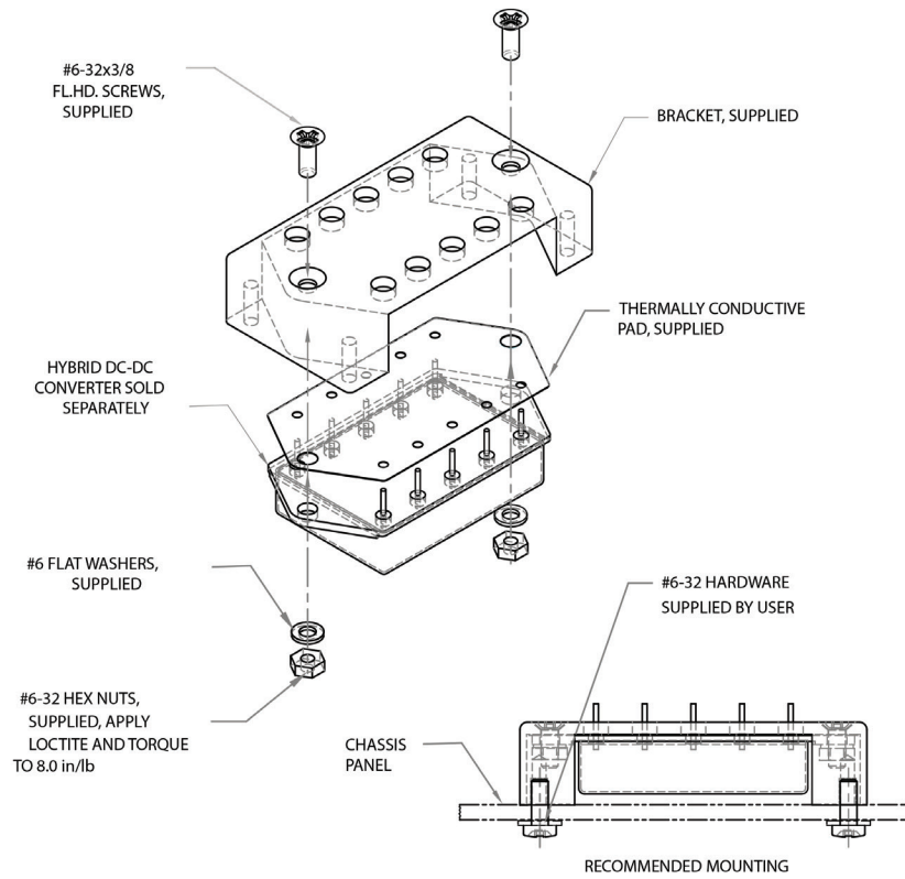
Typical Inverted Mounting Assembly Drawing
