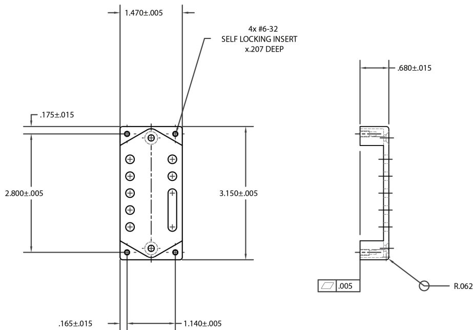
Typical Inverted Mounting Assembly Drawing
